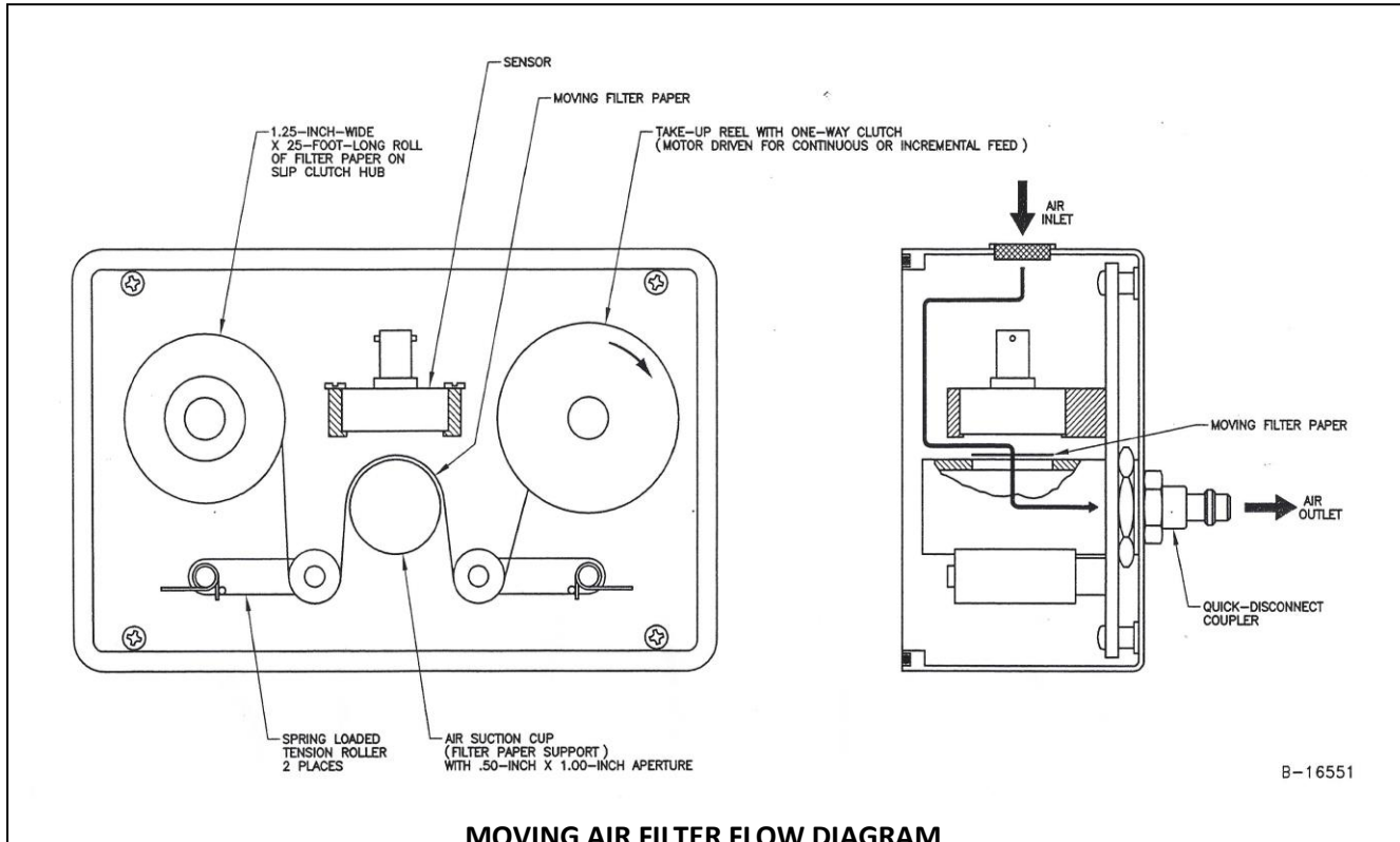
MOVING AIR FILTER FLOW DIAGRAM
